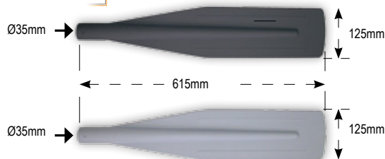
Blade for Paddles (50992-50995)
