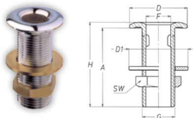
Through Hull Outlet, Chromium Plated Brass
