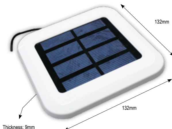
Solar Cell for Autonomous Solar Powered Fan
