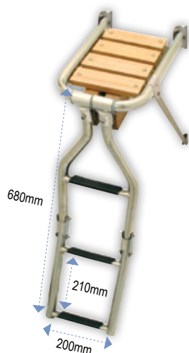
Wooden Platform with Inox 316 Ladder
