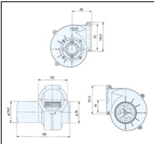
Electric Bilge Blower
