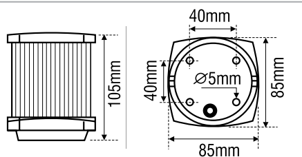
CLASSIC LED 20 Bulb (BAY15D), 12/24V
