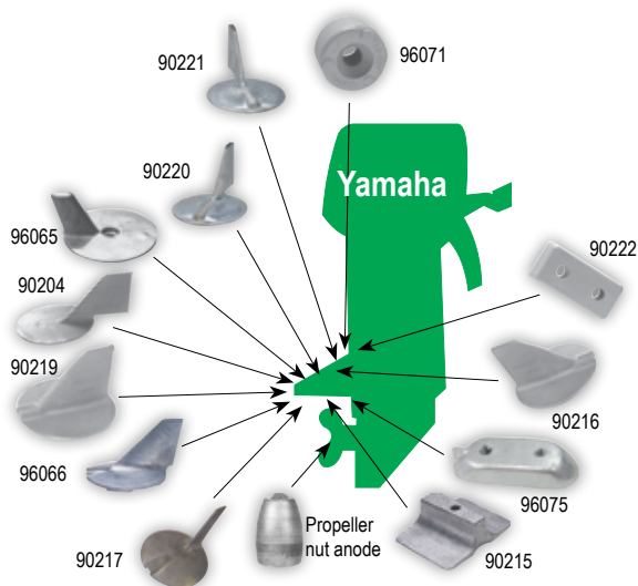
Anodes for Outboard Yamaha Engines
