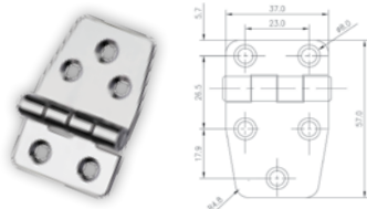
Hinge, Right, Inox 316
