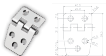
Hinge, Reversed, Inox 316
