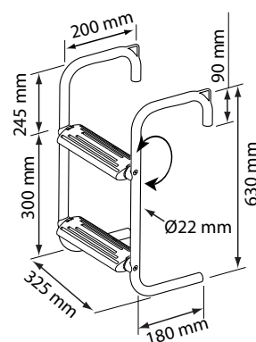
Raft Ladder, 2 Steps, Inox 316
