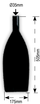
Paddle Blade, Ø35mm, 385gr, Black
