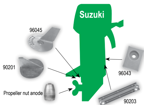
Anodes for Outboard Suzuki Engines
