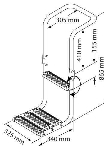
Immersed Platform Ladder, Inox 316
