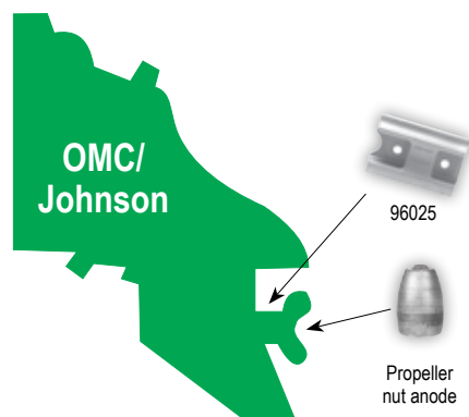
Anode for In/Outboard OMC/Johnson Engines
