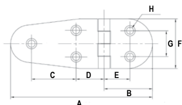
Hinge, Right, Inox 316
