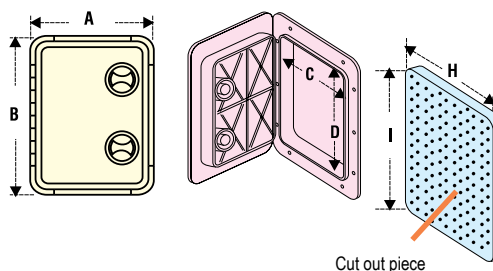
INDUSTRIAL Access Hatch UV-resistant PP (polypropylene)
