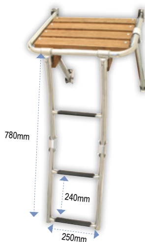
Wooden Platform with Folding Inox 316 Ladder
