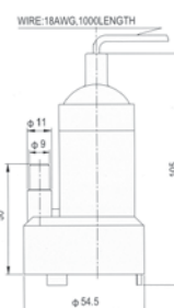
Water Pump for Tanks 160GPH, 12V, 2,5A
