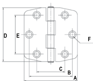
Hinge, Right, Inox 316
